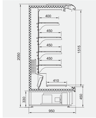
Fulya / Jonquil 950/2050
