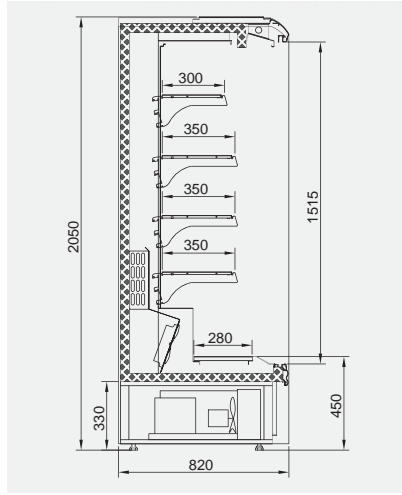
Fulya / Jonquil 820/2050
